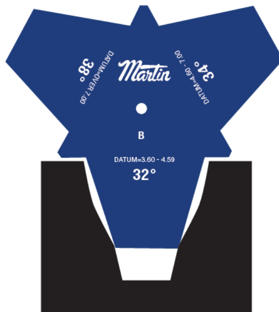
Worn Sheave (Dished Out)
