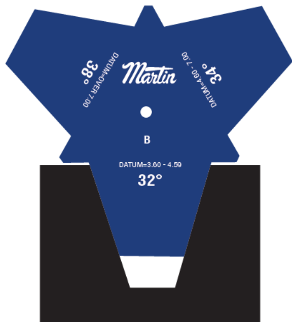
Normal Sheave (Uniform Angle)
